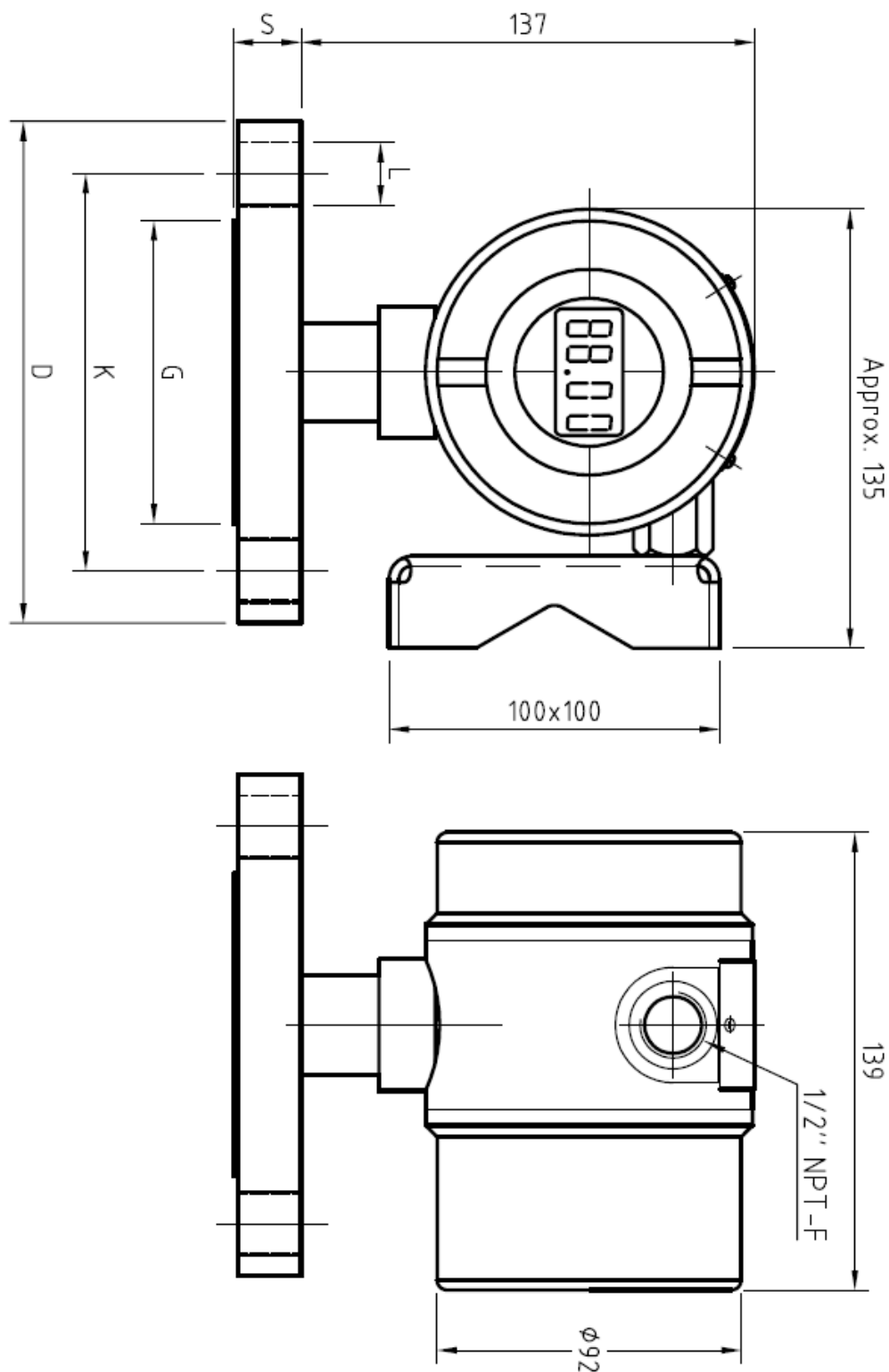
Figura 5 – Flanged connections UNI, ASME etc.
